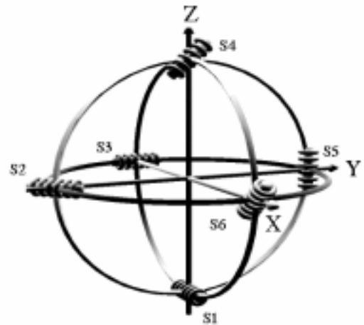
Fig. 1: Spherical placement of the 6 transmitter coils.
